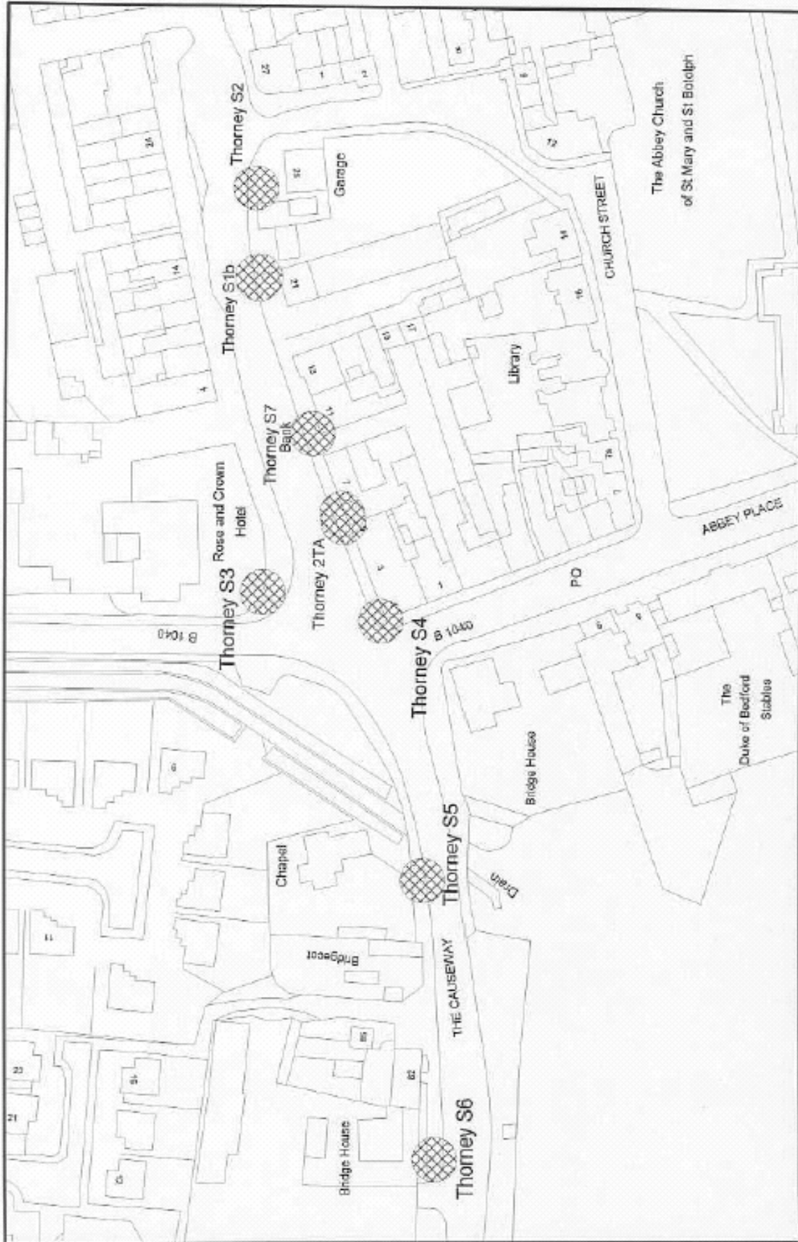
Figure 13. NO2 monitoring locations in Thorney
