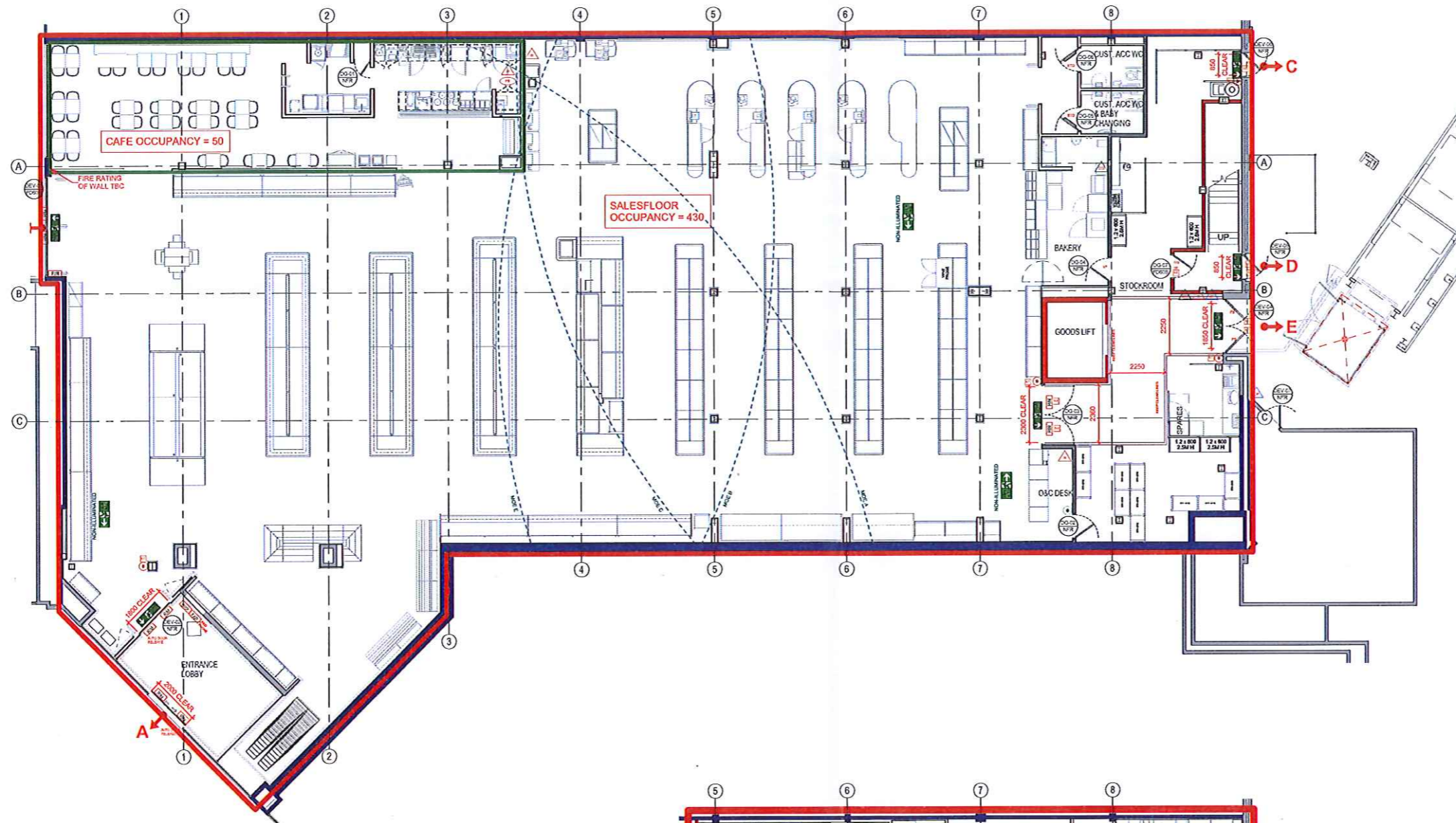
1 GROUND FLOOR LICENCING PLAN 1:100
