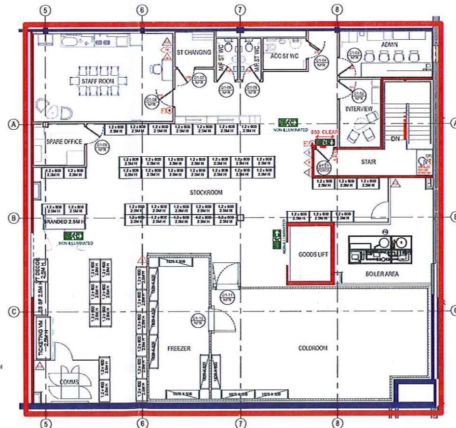
2 MEZZANINE FLOOR LICENCING PLAN 1:100
